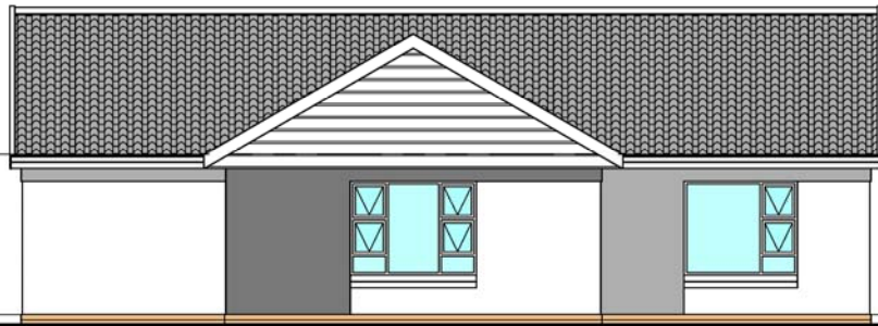
NORTH ELEVATION SCALE 1 : 100 ON A3
