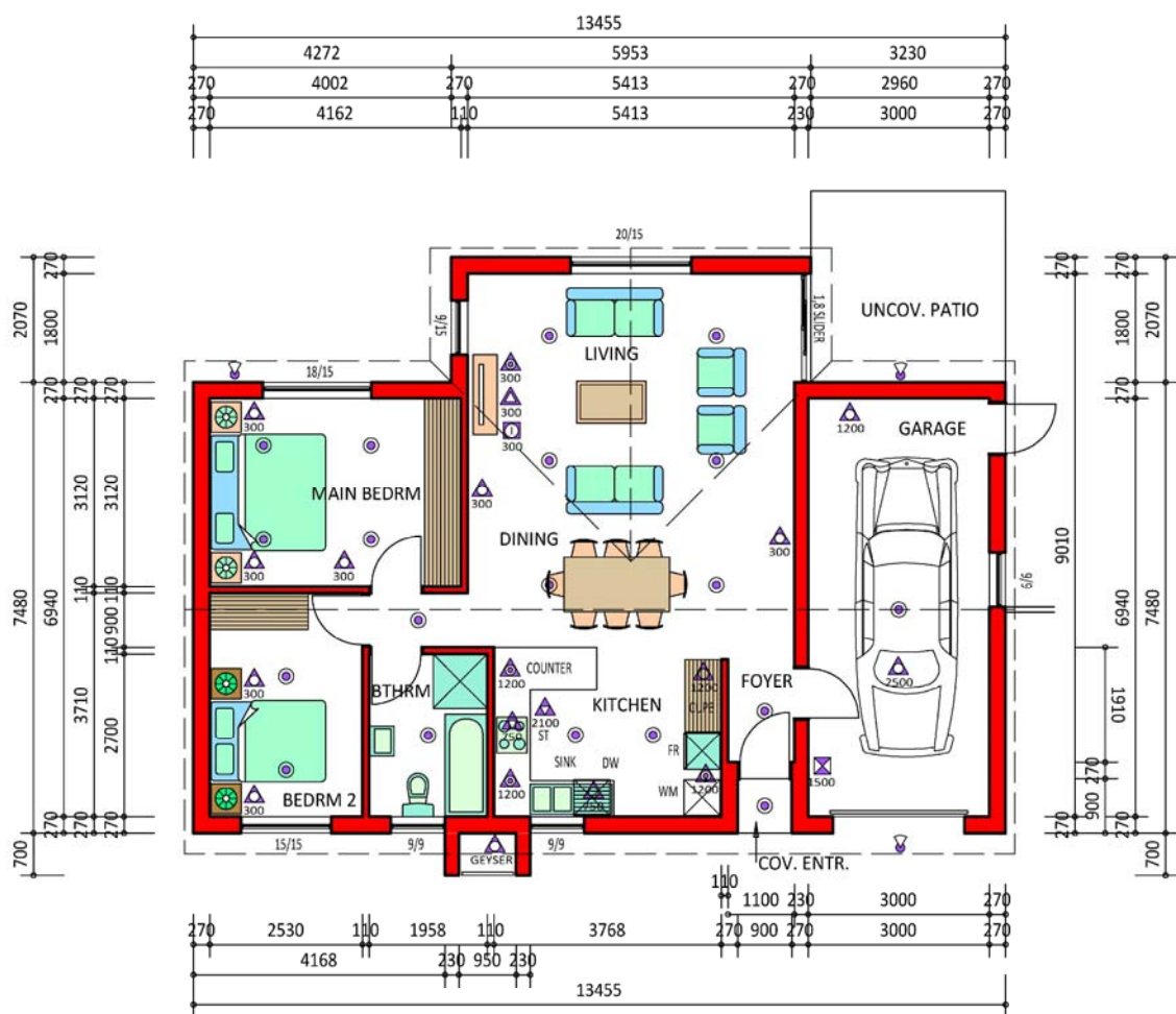
GROUND STOREY PLAN SCALE 1 : 100 ON A3
