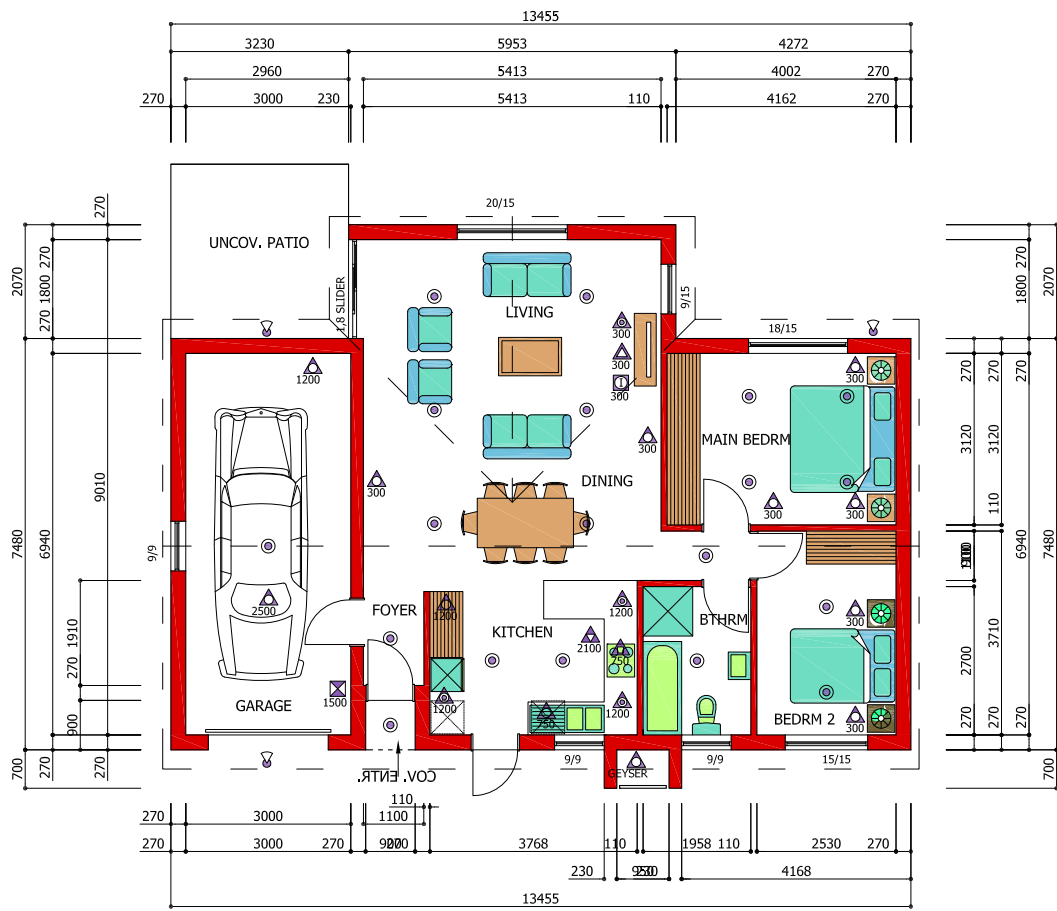
GROUND STOREY PLAN SCALE 1 : 100 ON A3
