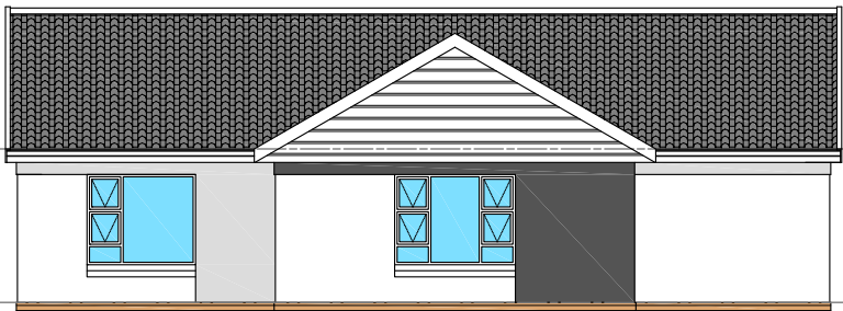
NORTH ELEVATION SCALE 1 : 100 ON A3
