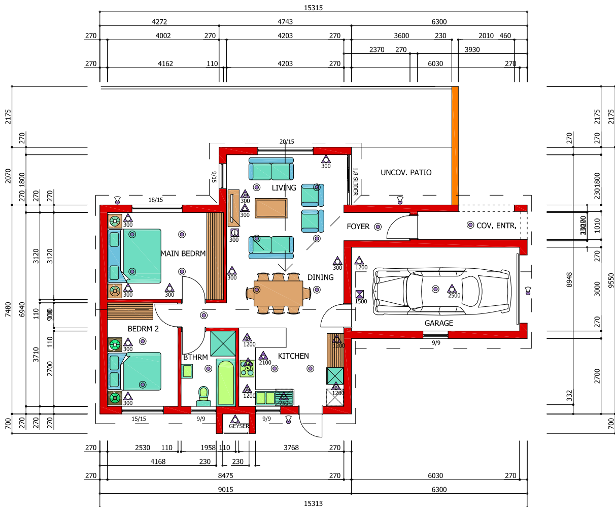
GROUND STOREY PLAN SCALE 1 : 100 ON A1
