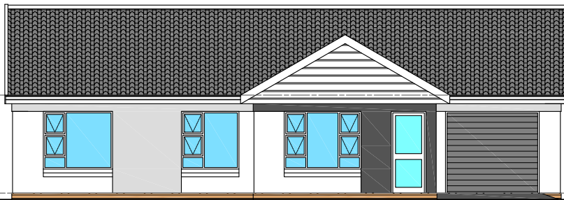
STREET ELEVATION SCALE 1 : 100 ON A3
