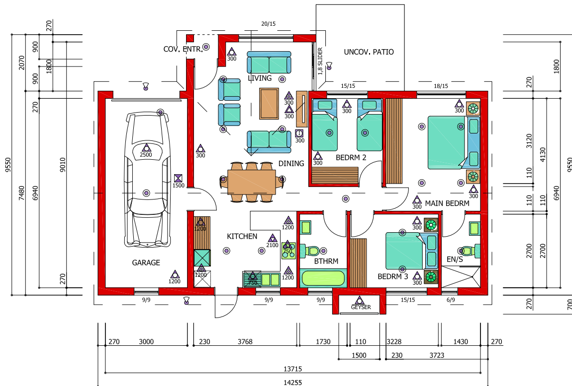
GROUND STOREY PLAN SCALE 1 : 100 ON A3
