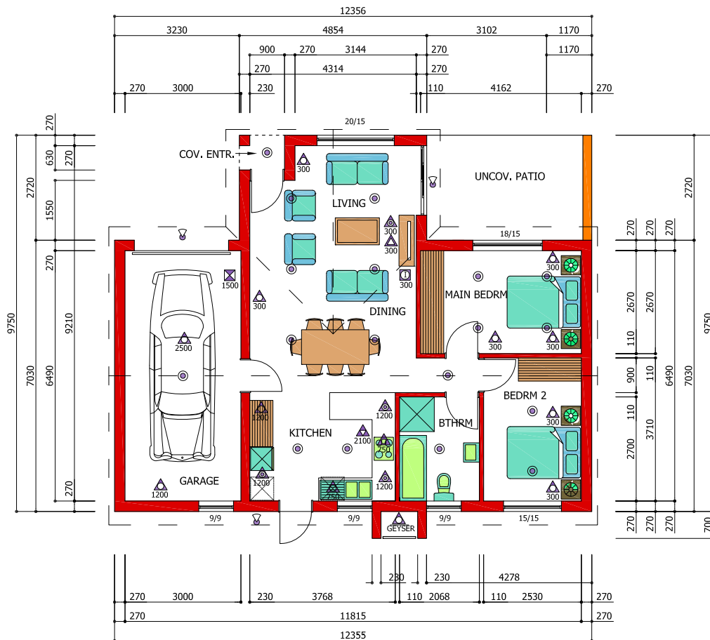
GROUND STOREY PLAN SCALE 1 : 100 ON A3
