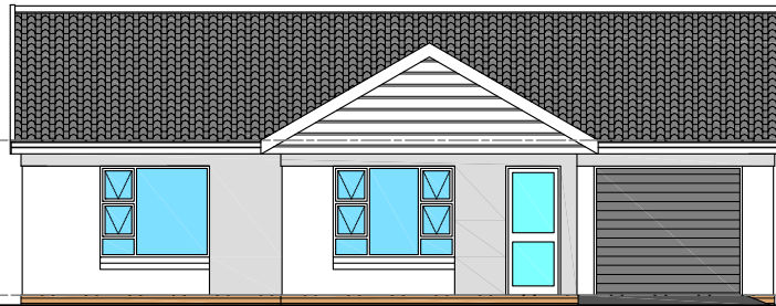
STREET ELEVATION SCALE 1 : 100 ON A3
