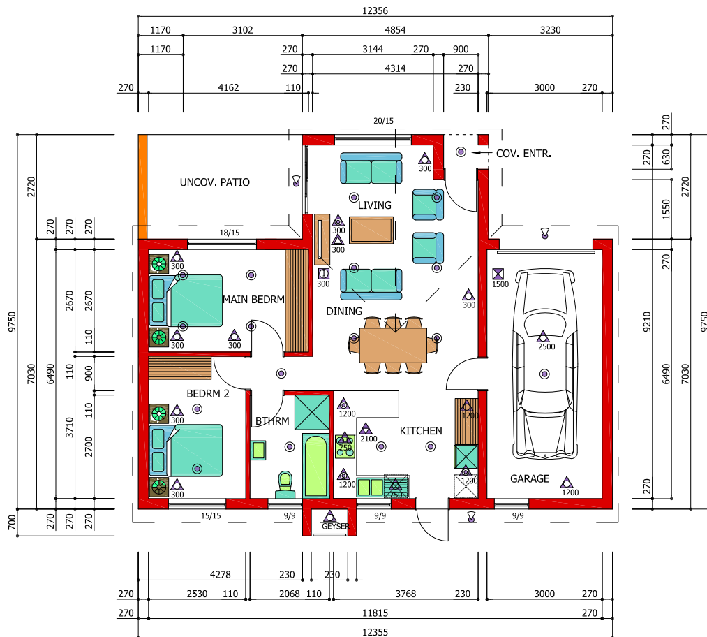
GROUND STOREY PLAN SCALE 1 : 100 ON A3
